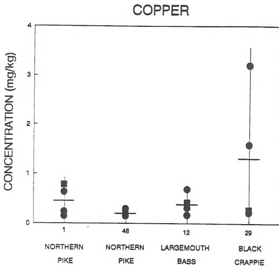
Figure 11. Comparison of replicate analyses from the same fish fillet. Squares represent the value of the initial determination while the circles represent copper from randomly selected tissue samples. Mean concentration (horizontal bar) and 95% confidence intervals are shown for the four samples.
